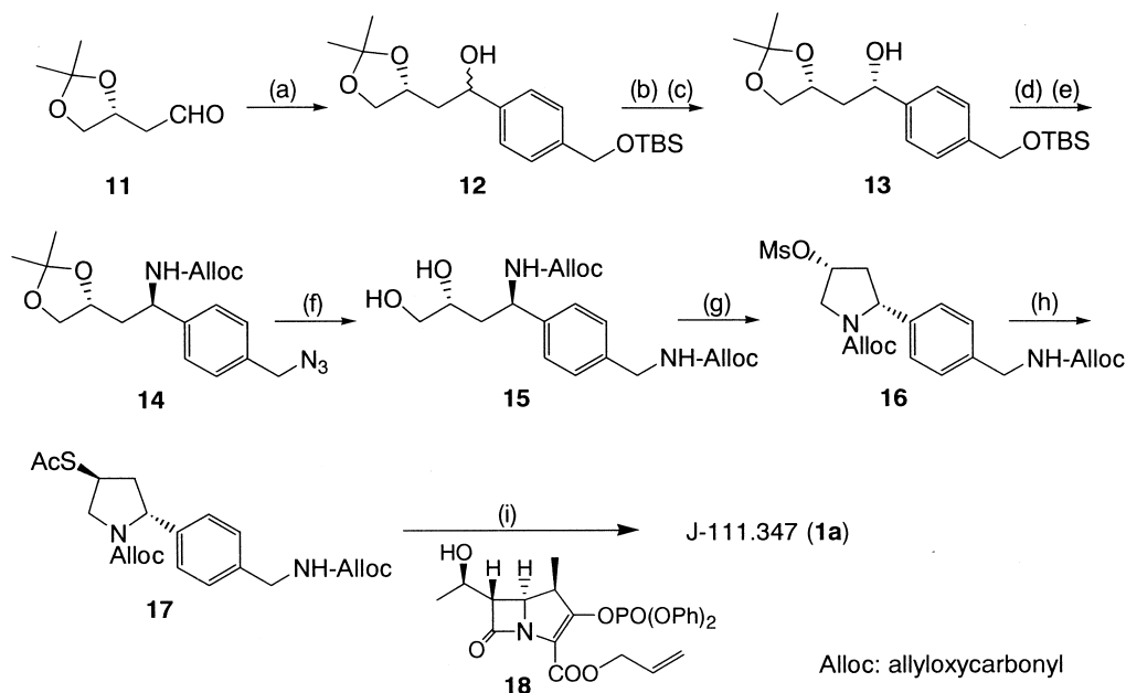
Scheme 1. Reagents; (a) 1-bromo-4-( tert -butyldimethylsilyloxy)methylbenzene, n -BuLi, THF, -70^{\circ}\text{C} , 88%, (b) TPAP, NMO, molecular sieve 4Å, \text{CH}_2\text{Cl}_2 , 0^{\circ}\text{C} , 88%, (c) \text{LiAlH}_4 , LiI, THF, -78^{\circ}\text{C} , 76%, (d) i: DEAD, \text{PPh}_3 , DPPA, THF, 0^{\circ}\text{C} , 86%; ii: \text{PPh}_3 , THF- \text{H}_2\text{O} , r.t.; iii: TEA, Alloc-Cl, THF, 0^{\circ}\text{C} , 90%, (e) i: n -Bu _4 NF, THF, 0^{\circ}\text{C} , 98%; ii: TEA, MsCl, \text{CH}_2\text{Cl}_2 , 0^{\circ}\text{C} ; iii: \text{NaN}_3 , DMF, r.t., 91%, (f) i: \text{PPh}_3 , THF- \text{H}_2\text{O} , r.t.; ii: TEA, Alloc-Cl, 0^{\circ}\text{C} ; iii: HCl-MeOH, 78%, (g) i: TEA, MsCl, \text{CH}_2\text{Cl}_2 , 0^{\circ}\text{C} ; ii: t -BuOK, THF, -20^{\circ}\text{C} , 97%, (h) AcSK, DMF, 65^{\circ}\text{C} , 86%, (i) i: NaOH, 0^{\circ}\text{C} ; ii: i -Pr _2 NEt, 18 , \text{CH}_3\text{CN} , 0^{\circ}\text{C} , 65%; iii: (\text{PPh}_3)_2\text{PdCl}_2 , n -Bu _3 SnH, \text{H}_2\text{O} , \text{CH}_2\text{Cl}_2 , 72%.
