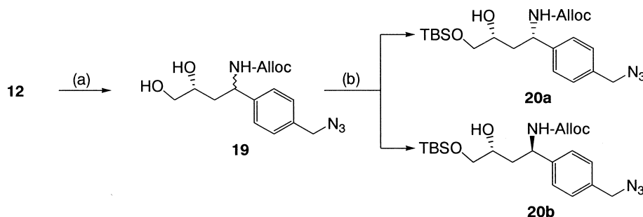
Scheme 2. Reagents; (a) i: DEAD, \text{PPh}_3 , DPPA, THF, 0^{\circ}\text{C} ; ii: \text{PPh}_3 , THF- \text{H}_2\text{O} , r.t.; iii: TEA, Alloc-Cl, THF, 0^{\circ}\text{C} ; v: TEA, MsCl, \text{CH}_2\text{Cl}_2 , 0^{\circ}\text{C} ; vi: \text{NaN}_3 , DMF, r.t.; vii: p -TsOH, MeOH, r.t., (b) TBS-Cl, imidazole, \text{CH}_2\text{Cl}_2 , r.t., 20a : 29.8%, 20b : 40.5%.
